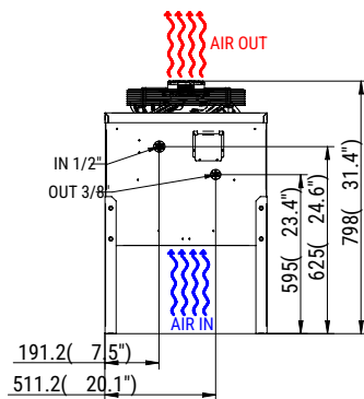
FRONTAL VIEW
