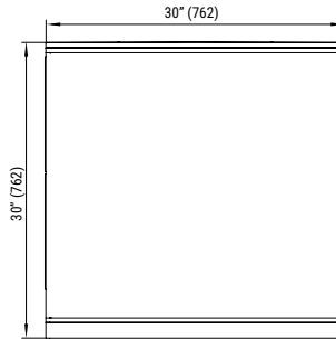
FRONTAL VIEW
