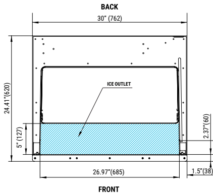
CENTRAL CROSS SECTION VIEW OF THE BASE
